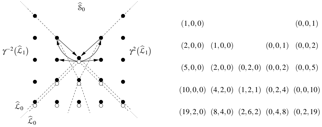
FIGURE 5. A schematic illustration of the states of the staggered module \widehat{S}_0 . We indicate the composition factors \gamma^{-2}(\widehat{\mathcal{L}}_1) , \widehat{\mathcal{L}}_0 and \gamma^2(\widehat{\mathcal{L}}_1) with dashed boundary lines (left) and the multiplicities of a few of the weight spaces (right). The latter are separated into those for each composition factor (the order is as above) with the multiplicities for \widehat{\mathcal{L}}_0 doubled (as it appears twice as a factor). At left, we split the weight spaces to distinguish the two \widehat{\mathcal{L}}_0 factors (as in Figure 4, the L_0 -eigenstates appear above their Jordan partners). We also indicate with arrows a few fundamental actions which define the indecomposable structure.
