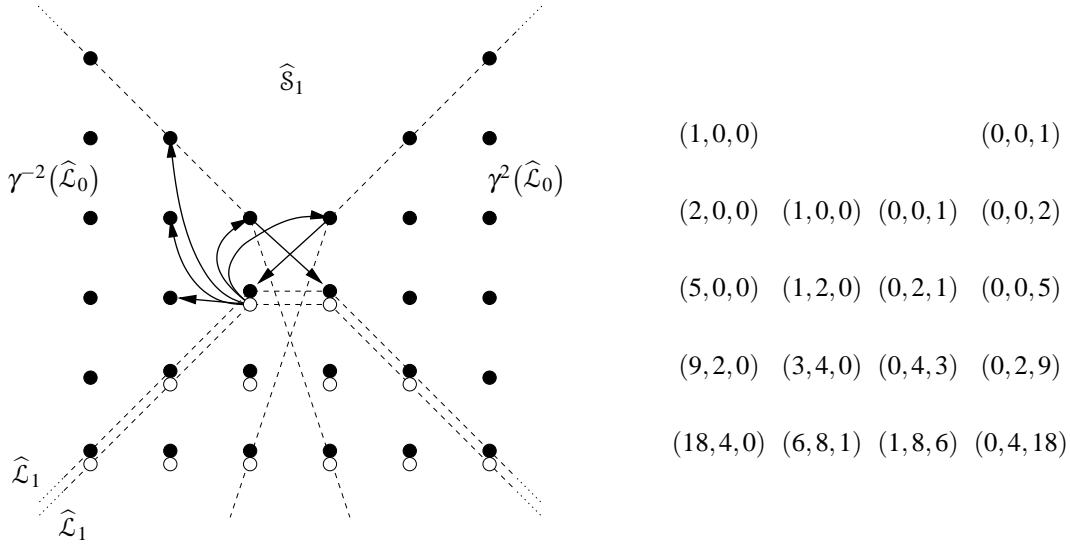
FIGURE 7. Schematic illustrations of the states and multiplicities of the staggered module \widehat{\mathcal{S}}_1 , following the conventions established for Figure 5. The multiplicities are for the composition modules \gamma^{-2}(\widehat{\mathcal{L}}_0) , \widehat{\mathcal{L}}_1 (doubled) and \gamma^2(\widehat{\mathcal{L}}_0) . As before, we indicate with arrows a few fundamental actions which result from the indecomposable structure.
