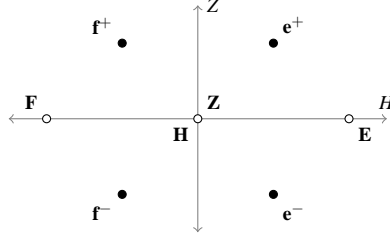
FIGURE 3. The weights ( \mathbf{H} - and \mathbf{Z} -eigenvalues) (H, Z) of the simple Lie superalgebra \mathfrak{sl}(2|1) , labelled by the corresponding weight vectors. White weights are bosonic and black weights are fermionic.
