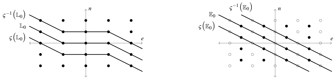
FIGURE 1. Schematic illustrations of the possible spectra of the proposed logarithmic and non-logarithmic \widehat{\mathfrak{gl}}(1|1) -theories. At left is the possible spectrum of the atypicals \widehat{\mathcal{A}}_{n,e} in both (and for the logarithmic theory, the indecomposables \widehat{\mathcal{P}}_{n,e} too). At right is the possible spectrum of typicals \widehat{\mathcal{T}}_{n,e} in the logarithmic theory (the atypical points are marked in white for comparison). Modules corresponding to points on the same line yield the same coset module as indicated.
