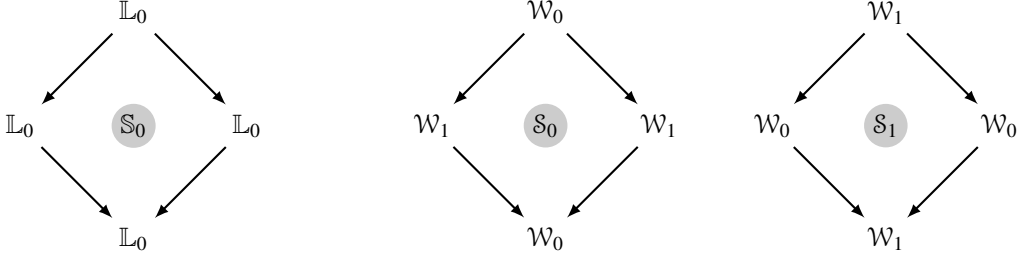
FIGURE 4. The Loewy diagrams for the socle series of the indecomposable symplectic fermion module \mathbb{S}_0 (left) and the indecomposable \mathfrak{W}(1,2) -modules \mathcal{S}_0 and \mathcal{S}_1 (right). In each case, the non-diagonalisable action of L_0 maps the top factor (the head) onto the bottom factor (the socle).
