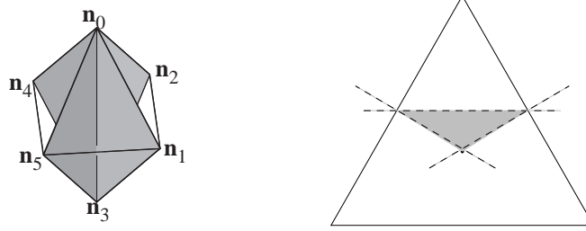
FIGURE 7. Decomposition into ideal tetrahedra and corresponding parameter cell.
