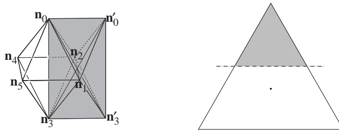
FIGURE 8. Decomposition into square-based pyramids and corresponding parameter cell.
