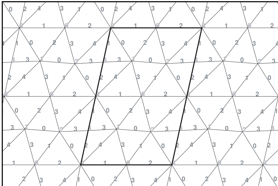
FIGURE 3. The cusp triangulation of M = M_{\varphi_w} where w = LRRLR . The triangulation of M has five edges, labelled 0-4, which appear as both edges and vertices of the cusp triangulation.
