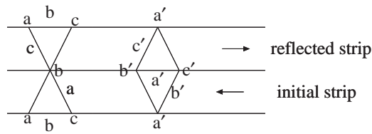
FIGURE 4. Edge identifications in strips of T_0 .
