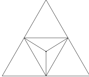
FIGURE 9. All parameter cells for canonical decompositions of the Borromean rings complement
