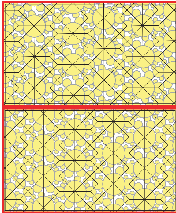
FIGURE 1. The maximal horoball packing and canonical cell decomposition as seen from the cusps of manifolds m137 and m138 .
