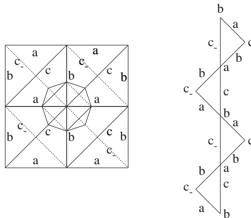
FIGURE 2. The chain of triangles around a cusp coming from one tetrahedron.
