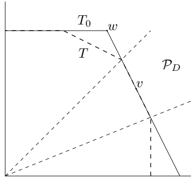
FIGURE 5. T_0 is a partially computed tilt polytope. The face of T_0 containing v \in \mathcal{P}_D has a vertex w not in \overline{\mathcal{P}_D} . Therefore D(w) gives another face of T .
