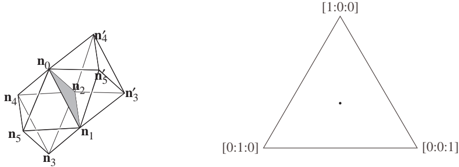
FIGURE 6. Initial cell decomposition of M into ideal octahedra and the corresponding projective parameter cell.
