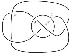
FIGURE 10. Complete the numbering indicated on the above two-component link to obtain the Dowker-Thistlethwaite code (6, -8) (-10, 14, -12, -16, -2, 4) .
