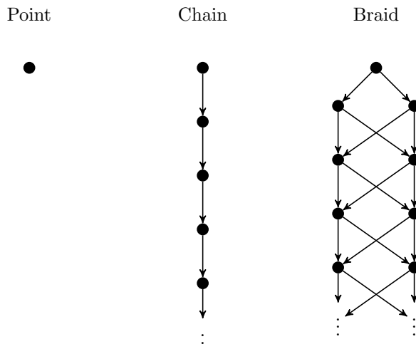
Figure E.1: The singular vector structure, marked by black circles, of Virasoro Verma modules for t \in \mathbb{Q}_+ . Arrows from one singular vector to another indicate that the latter may be obtained from the former by acting with Virasoro modes. The chain and braid structures have infinitely many singular vectors. The conformal dimensions of the singular vectors increase as one moves down.
