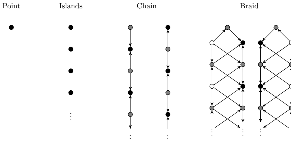
Figure E.3: The subsingular vector structure of Virasoro Feigin-Fuchs modules for t \in \mathbb{Q}_+ . Black circles represent the socle of the module, grey the second socle layer, and white the third. Each of the black circles corresponds to a singular vector and the top circle (of lowest conformal dimension) is always singular, but the rest are only subsingular. Arrows from one subsingular vector to another indicate that the latter may be obtained from the former via the Virasoro action. Note that the two braid diagrams that we have drawn are structurally identical. This repetition serves to indicate that the corresponding Feigin-Fuchs modules are not self-contragredient. The conformal dimensions of the subsingular vectors are chosen to increase as one moves down and to the right.
