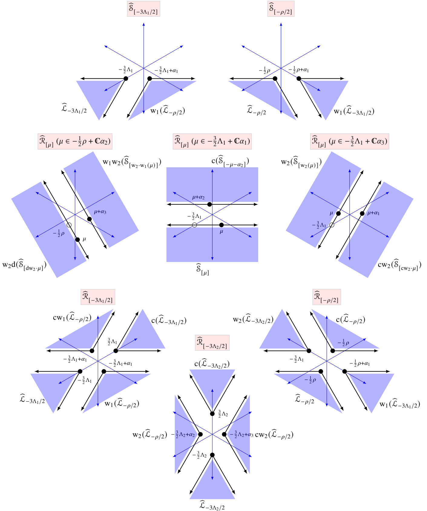
FIGURE 5. The degenerations (5.10) of the semirelaxed A_2(3, 2) -modules (top), the generic degenerations (5.11) of the relaxed A_2(3, 2) -modules \widehat{\mathcal{R}}_{[\mu]} , \mu \in \text{sing}(-\frac{3}{2}\Lambda_1) , (middle) and the special degenerations (5.12) of the relaxed A_2(3, 2) -modules (bottom). In each case, the degeneration is illustrated by the (convex hulls of the) weights of the direct summands and the black circles indicate representative weights of the summands.
