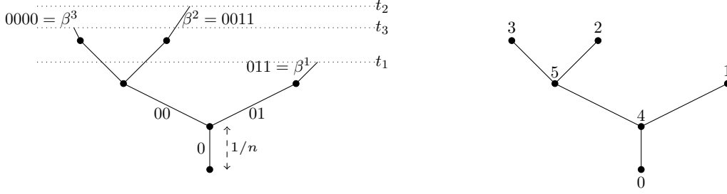
Figure 7: On the left is (part of) a GW tree with \beta^1, \beta^2, \beta^3 indicated. Here |\beta^1| = |\beta^5| = 2 , |\beta^2| = |\beta^3| = 3 , and |\beta^4| = 1 , and this contributes to (2.21) when t_2, t_3 \in [3/n, 4/n) and t_1 \in [2/n, 3/n) as depicted. On the right is the corresponding tree shape. The edge lengths associated to the latter are determined by taking differences of the u_e , where u_4 = 1/n , u_5 = 2/n , u_1 = t_1 , u_2 = t_2 , u_3 = t_3 .
