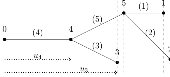
Figure 5: A depiction of a shape F \in \Sigma_3 with vertex labels above vertices and edge labels in brackets. The set of edges in the path from vertex 0 to vertex 1 is \mathcal{E}_1(F) = \{1, 4, 5\} . Variables u_i are associated to each of the vertices i , describing a ‘length’ from 0 to i , to form \mathcal{T}(F, \vec{u}) . Differences in these u_i are then the “edge lengths”.
