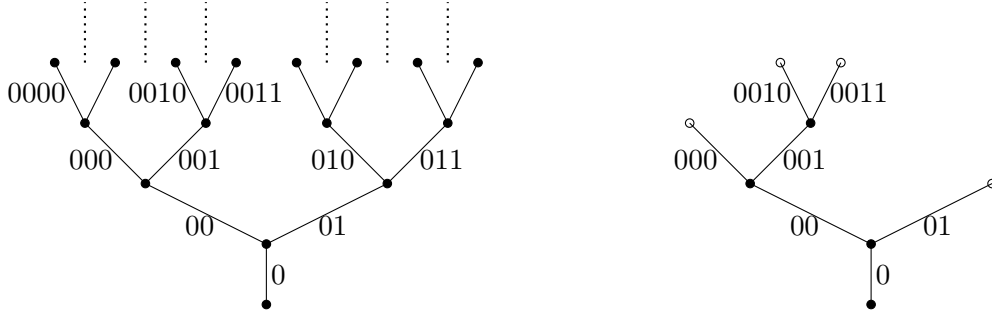
Figure 3: On the left is the index set I drawn (with labels as edges) up to and including generation 3. On the right is an example of a GW tree (with edge labels \alpha ), where e^\alpha = 0 for all \alpha \in \{000, 0010, 0011, 01\} , while e^\alpha = 2 for \alpha \in \{0, 00, 001\} .
