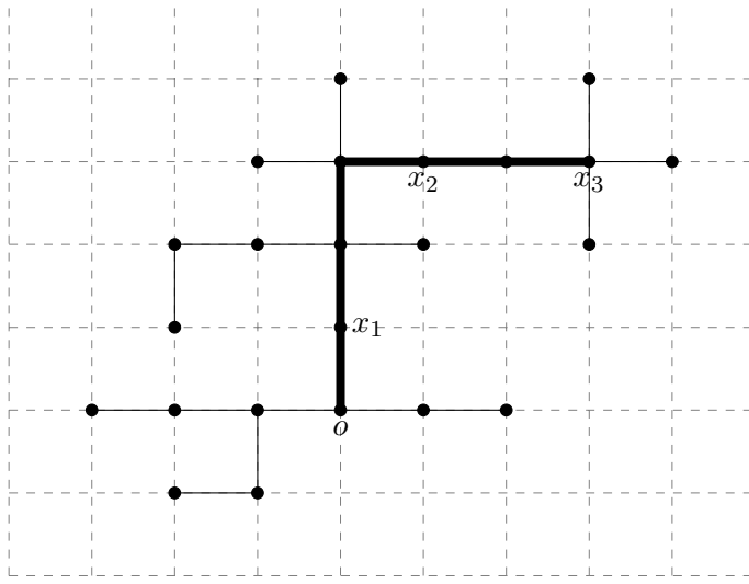
Figure 8: A depiction of the event in the detailed 1-particle function with n = 1 , t = 6 , s_1 = 1 and s_2 = 4 , with the path w.(6, x_3) in bold.
