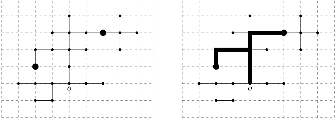
Figure 2: The MVP X_5^{(1)} assigns masses to points in the tree distance 5 from the root, while H_5^{(1)} assigns the same masses to paths in the tree leading to these points.
