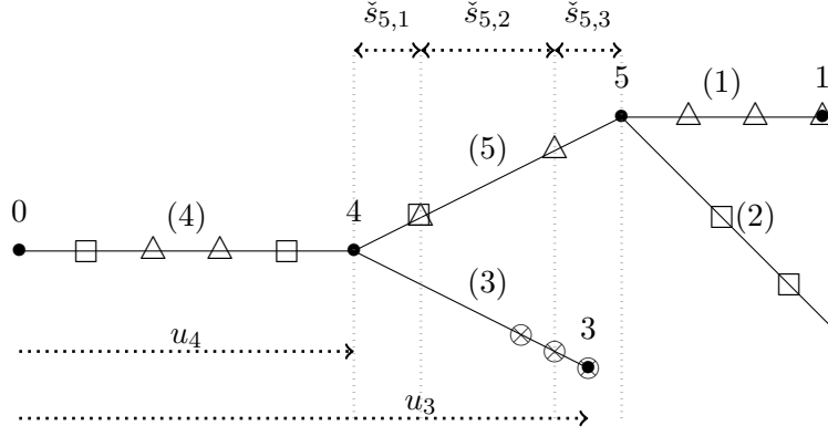
Figure 6: The tree \mathbb{T}(F, \vec{u}) together with times \mathbf{s} . The ( m^{(1)} = 7 ) \triangle symbols represent times s_1^{(1)}, \dots, s_7^{(1)} . Similarly \square symbols represent times s_j^{(2)} (with m^{(2)} = 6 ) and \otimes symbols represent times s_j^{(3)} (with m^{(3)} = 3 ) respectively. In this example there is one point (on edge 5) that is both square and triangle simultaneously. The ‘subinterval’ lengths \check{s}_{5,i} are indicated for edge 5.
