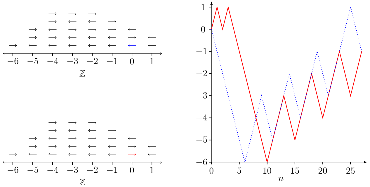
Figure 2: On the left are parts of arrow systems \mathcal{L} (top) and \mathcal{R} (bottom) with \mathcal{L} \subseteq \mathcal{R} , and on the right are the corresponding paths R_n (solid) and L_n (dotted). Here, |A_{R,26}| = 7 < 9 = |A_{L,26}| .
