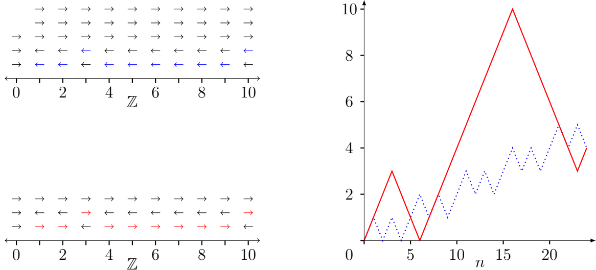
Figure 1: On the left are parts of the systems \mathcal{L} (top) and \mathcal{R}(3) (bottom) and on the right are their corresponding sequences R_n (solid) and L_n (dotted), defined in Section 4 such that \liminf n^{-1}L_n \geq \liminf n^{-1}R_n . Each site in \mathbb{N} appears five times in the sequence L and three times in the sequence R .
