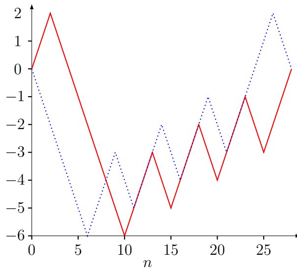
Figure 3: Paths R'_n (solid) and L'_n (dotted) with L'_n \preceq R'_n and |A_{R,28}| = 7 < 10 = |A_{L,28}| . The walks have visited each site the same number of times.
