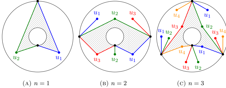
FIGURE 2. Hypermaps z^n + \frac{1}{z} , 1 \leq n \leq 3
