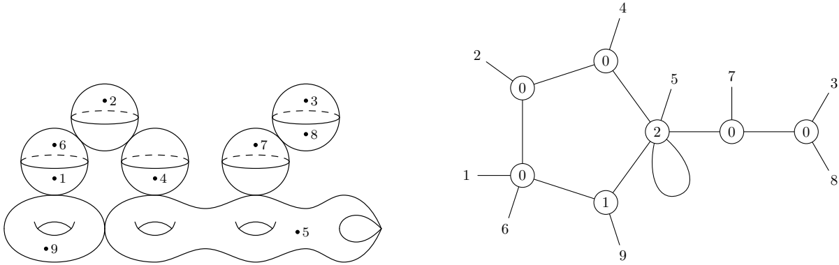
FIGURE 1. Dual graph of a stable curve.
